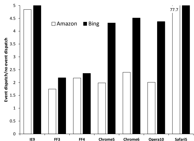
Figure 21. Cross-browser comparison. Impact of events on throughput. (number normalized to the replay without event processing; average over five runs; lower is better)
