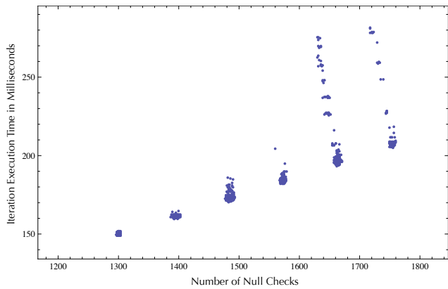
Figure 5. Correlation between number of null checks in an iteration and that iteration’s execution time in CDj.
