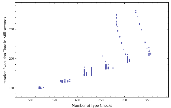
Figure 7. Correlation between number of type checks in an iteration and that iteration’s execution time in CDj.
