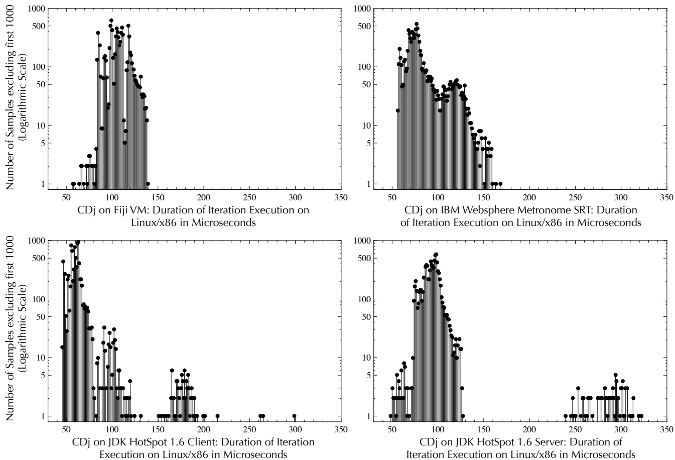
Figure 8. Histograms of iteration execution times for CDj on Linux/x86. Fiji VM achieves the best observed worst-case and has the tightest distribution of execution times – representing the best predictability. WebSphere SRT has a slightly better average performance but with a larger variance. Hotspot client and server have the best average-case performance but exhibit poor worst-case performance with outliers above 300 microseconds. We exclude the first 1,000 iterations from the measurements to avoid initialization bias.
