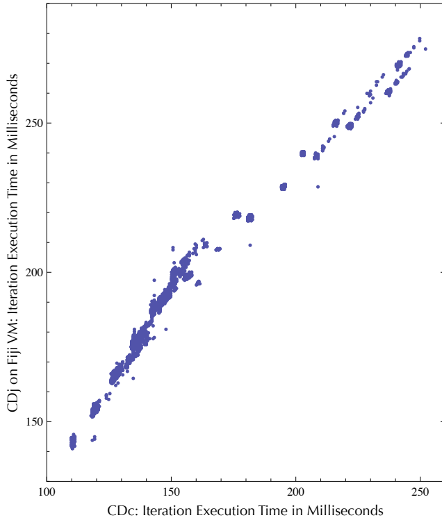
Figure 4. Execution time correlation between CDc and CDj.
