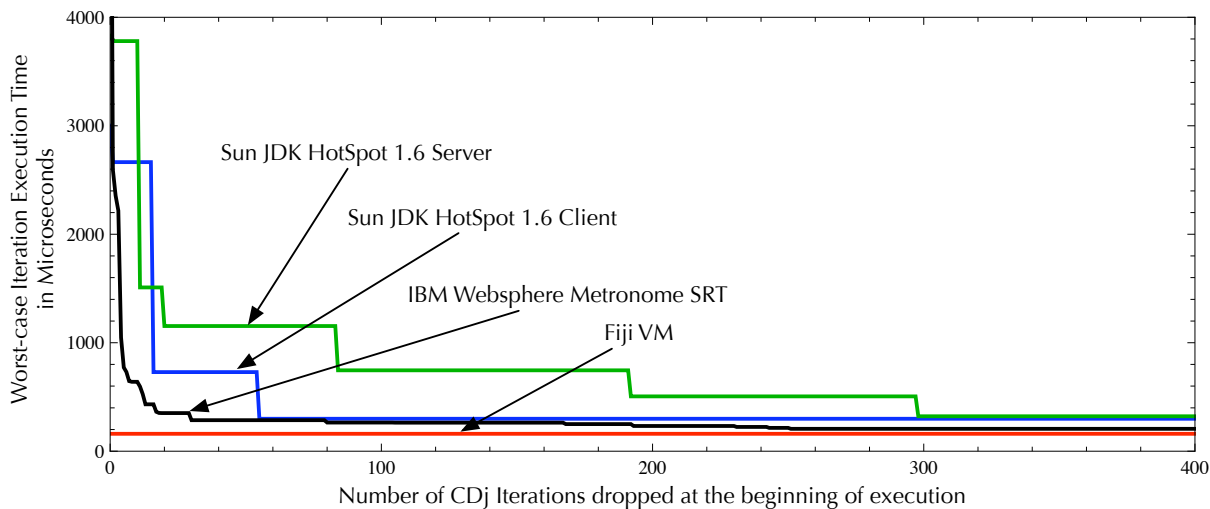
Figure 9. Start-up costs. The Y-axis shows the worst-case observed execution time, while the X-axis shows iterations dropped from the 10,000 performed for each VM. The initial iterations are dominated by the just-in-time compiler. This is particularly true for Hotspot server. WebSphere also has a JIT but it is tuned to stabilize faster. In comparison, the Fiji VM does not suffer from start-up jitter. If roughly 300 or more iterations are dropped, the JIT-based systems have a worst-case that approaches Fiji VM's. At that point the worst-case is dominated by garbage collection where the Fiji VM performs well due to its fully concurrent and slack-based collection strategy.
