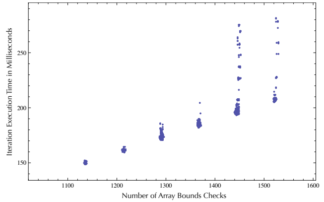
Figure 6. Correlation between number of array bounds checks in an iteration and that iteration’s execution time in CDj.
