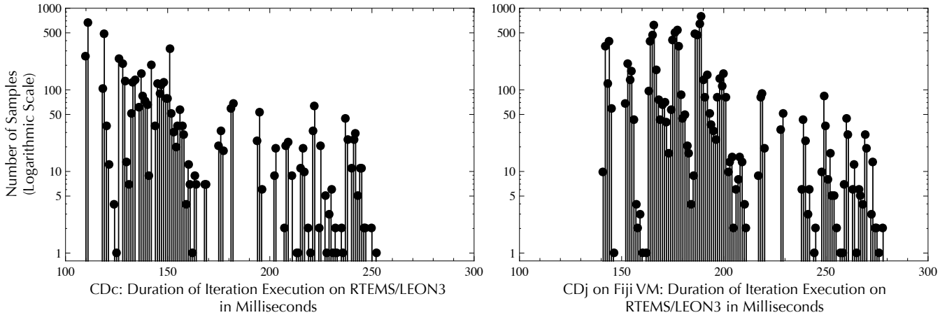
Figure 2. Histograms of iteration execution times for CDc and CDj on RTEMS/LEON3. Java’s worst observed case is 10% slower than C, and the median is 30% slower.
