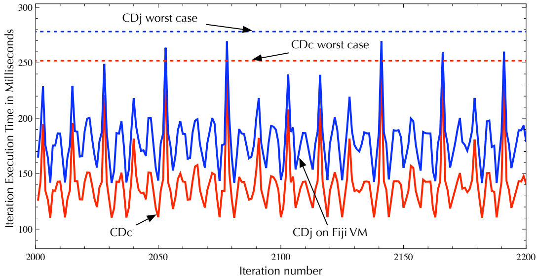
Figure 3. A detailed runtime comparison of CDc and CDj for 200 iterations. Java and C execution times are closely correlated. CDj is run with GC enabled. In 10,000 iterations there are 15 collections, but they never impact execution time.
