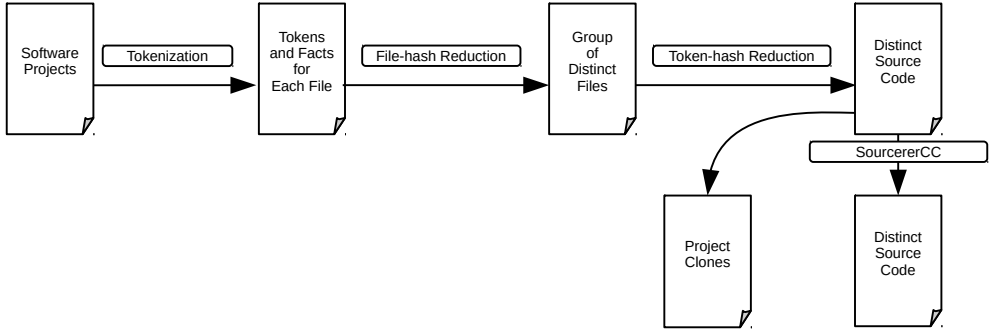
Fig. 3. Analysis pipeline.
